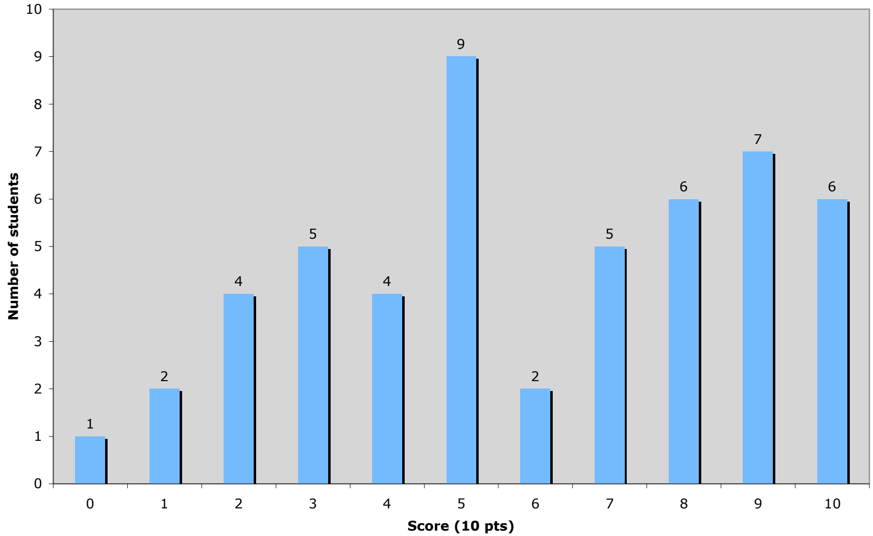
HW 7 Histogram
